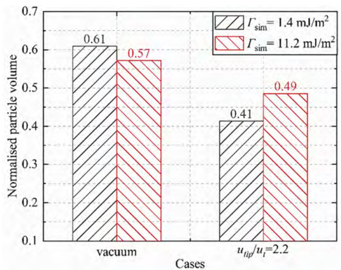
Fig. 12. Normalised particle volume in the cases of particles with surface energy of 1.4 \text{ mJ/m}^2 and 11.2 \text{ mJ/m}^2 .
