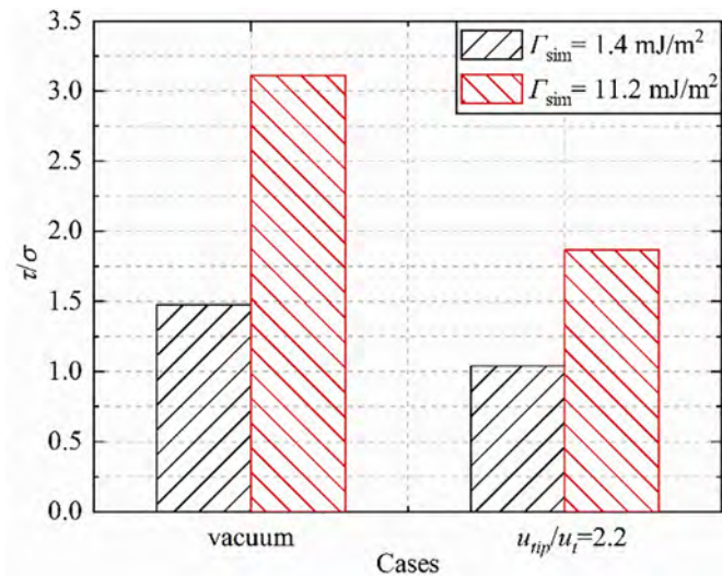
Fig. 14. Ratio of shear stress to normal stress for the particle flow in the gap region in the cases of particles with surface energy of 1.4 \text{ mJ/m}^2 and 11.2 \text{ mJ/m}^2 .
